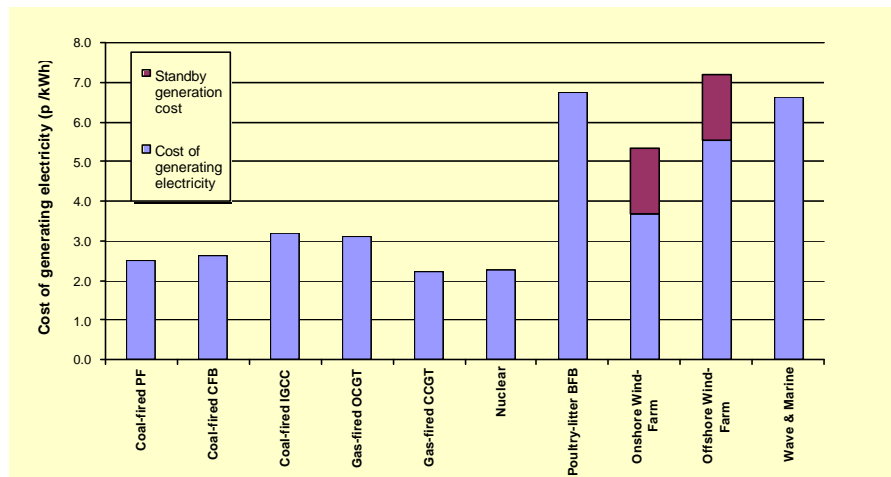
Figure 1 Cost of generating electricity (pence per kWh) with no cost of CO 2 emissions included.
