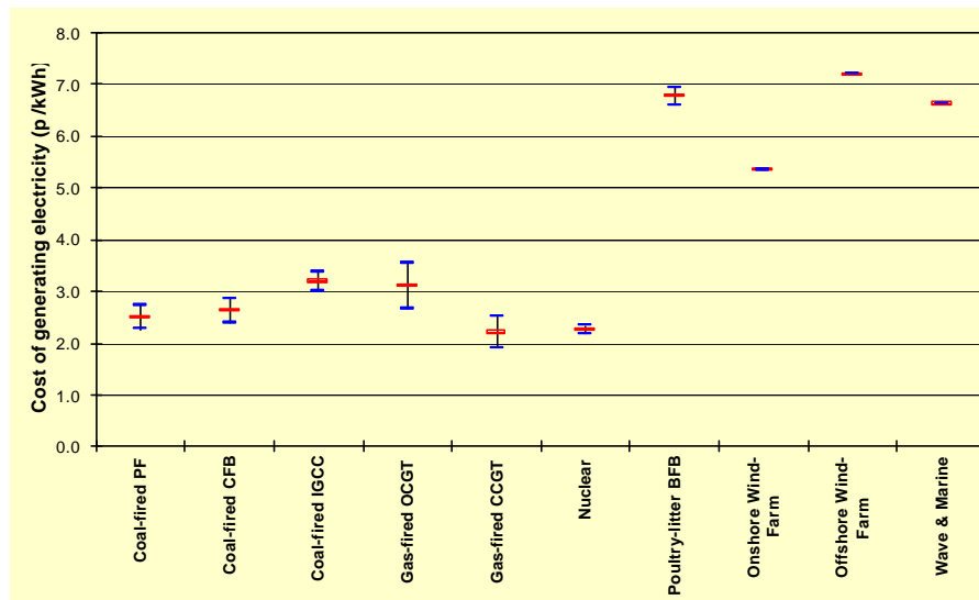
Figure 2 Effect of \pm 20\% change in fuel price on the cost of generating electricity
